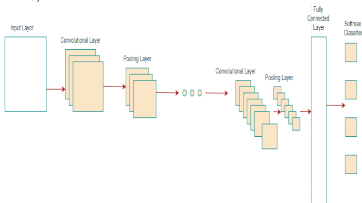
Fig. 1. Basic Structure of CNN
